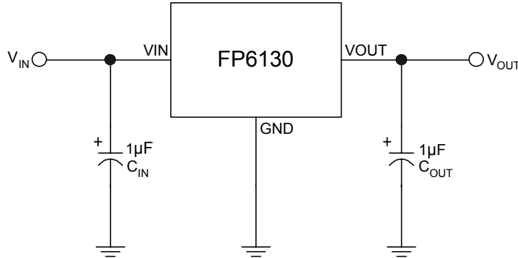
Figure 2. Typical Application Circuit of FP6130
