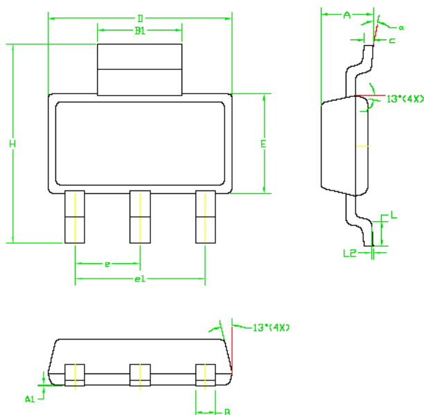
SOT-223 Package (Unit: mm)
