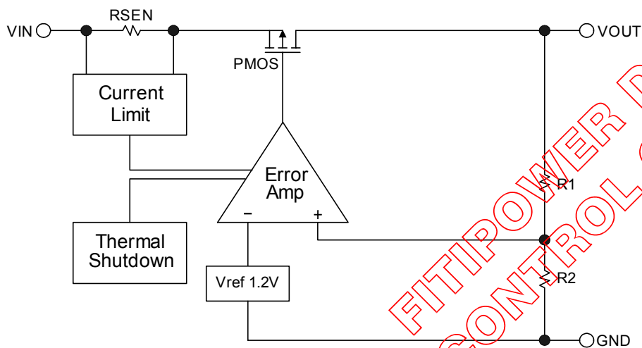
Figure 3. Block Diagram of FP6130
