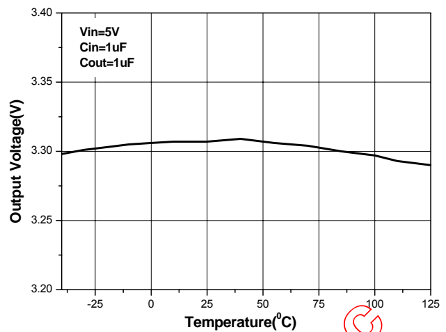
Figure 13. Temperature Stability
