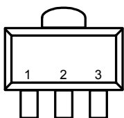
Figure 1. Pin Assignment of FP6130
