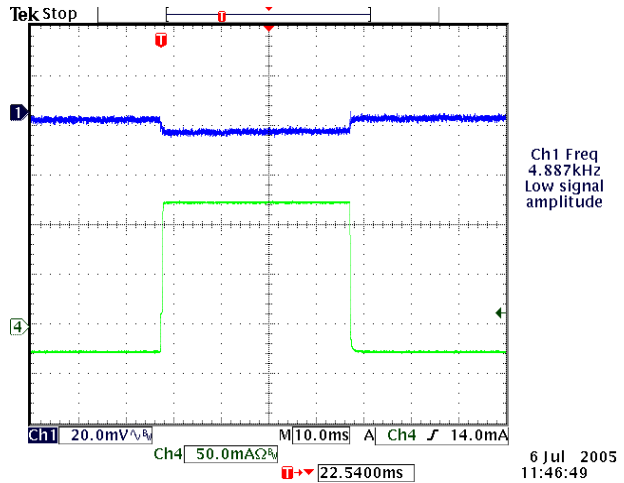
Figure 16. Load Transition Response
