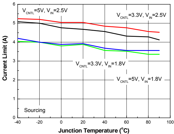
Figure 8. Current Limit vs. Junction Temperature
