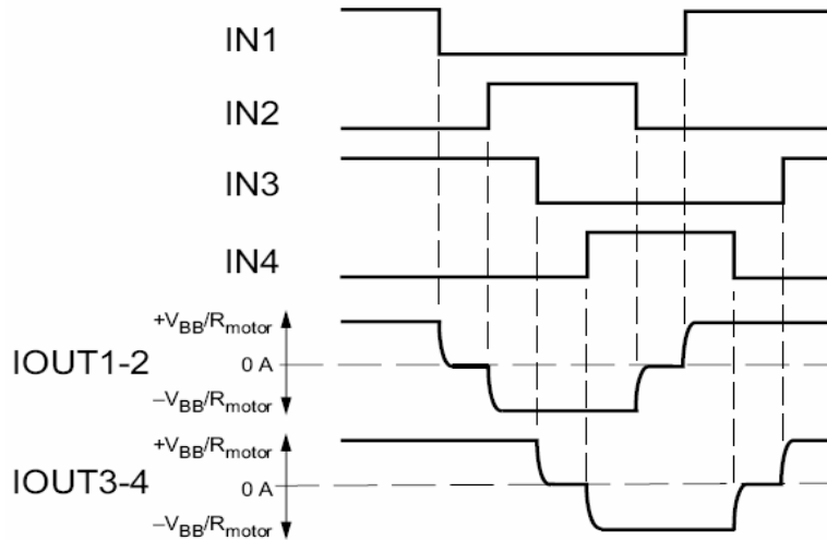
Figure 5d. Half step mode timing chart
