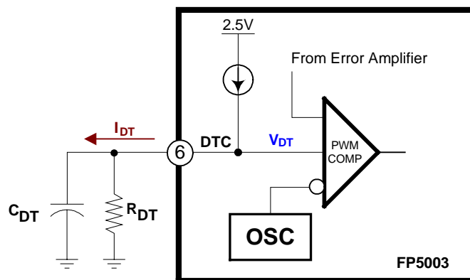
Figure 15. Soft-Start Circuit
