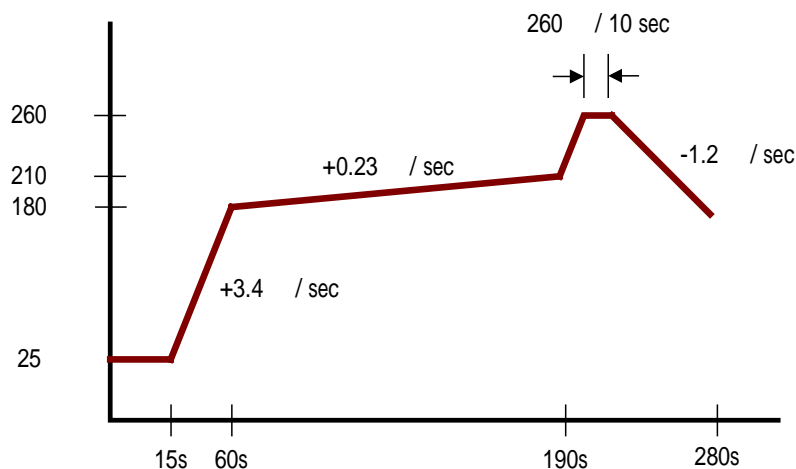
Lead Free Soldering Curve
