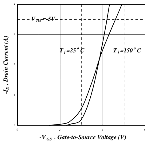
Fig 11. Transfer Characteristics
