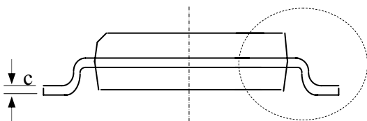
DETAIL A
