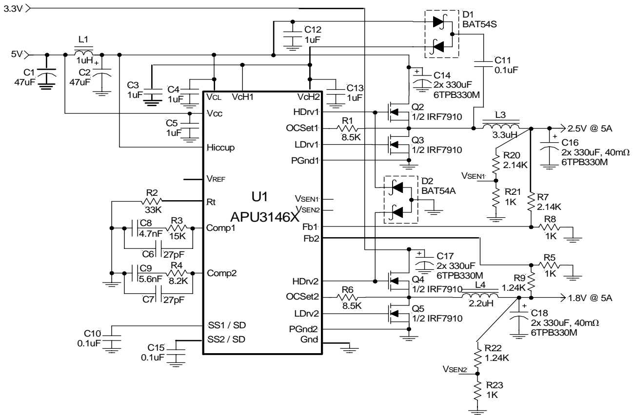
Figure 42 - Typical application of APU3146X. 5V to 2.5V and 3.3V to 1.8V inputs and two independent outputs.
