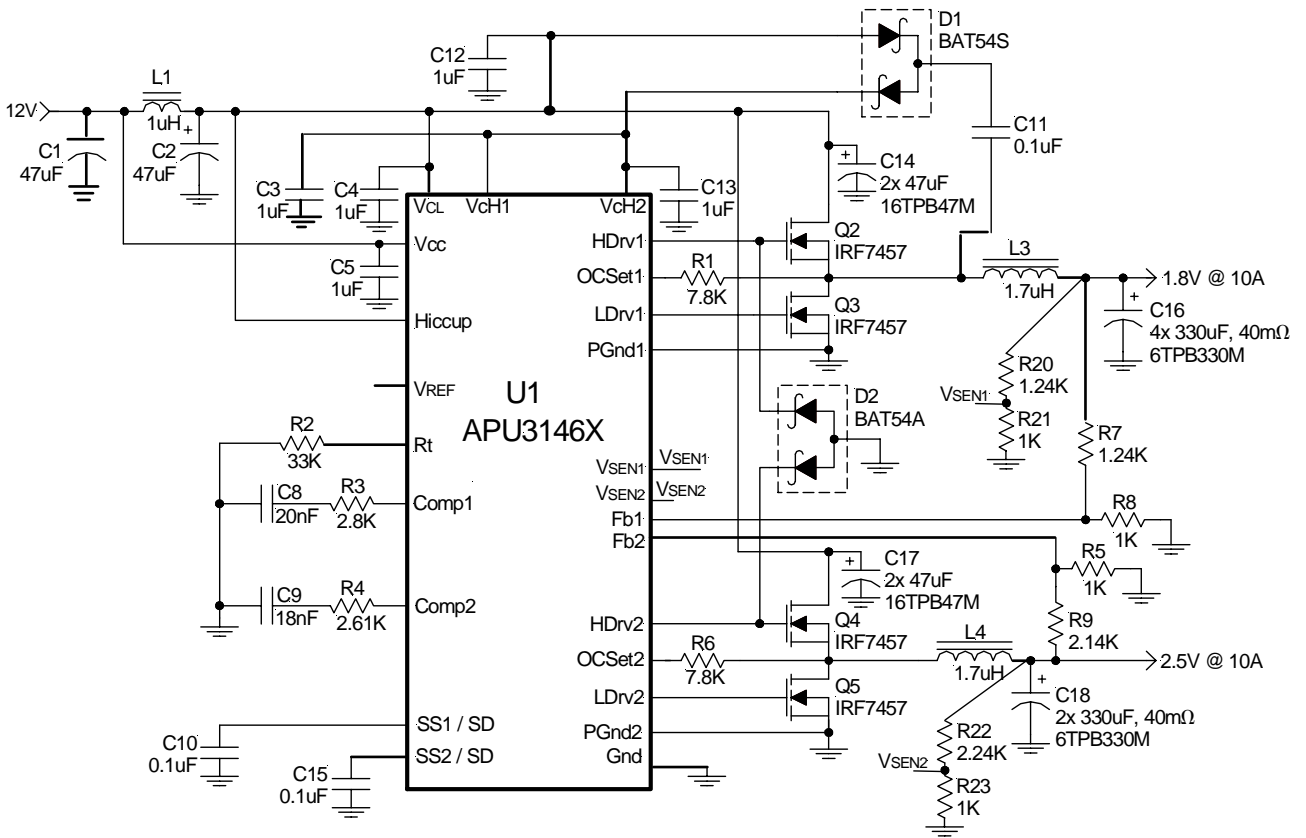
Figure 19 - Typical application of APU3146X 12V input and two independent outputs.
