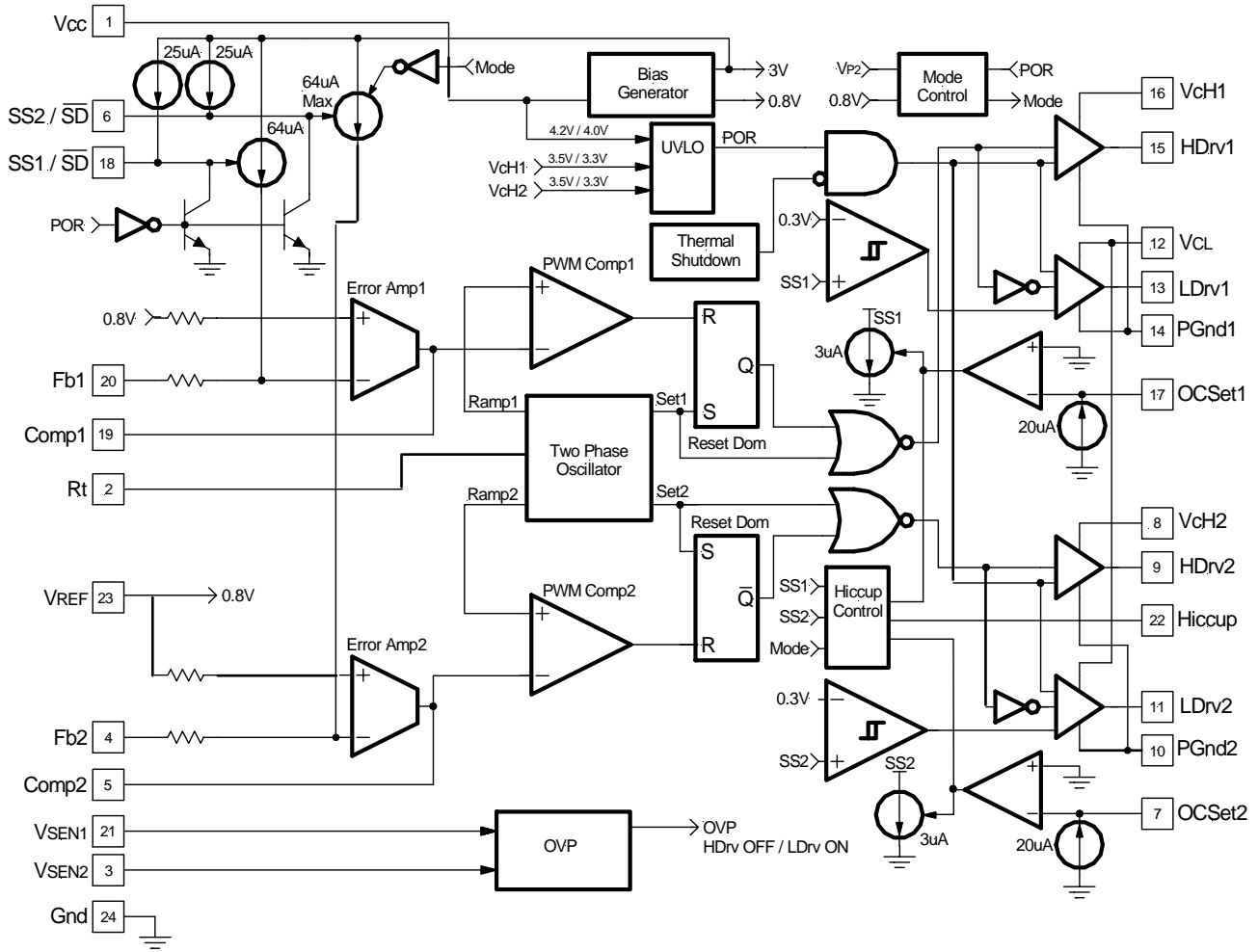
Figure 3 - Block diagram of APU3146X.
