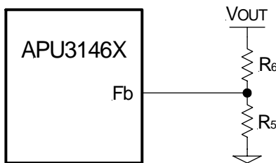
Figure 11 - Typical application of the APU3146X for programming the output voltage.
