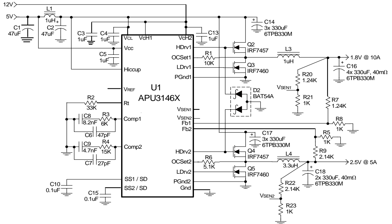
Figure 41 - Typical application of APU3146X. 5V input, 12V drive and two independent outputs.
