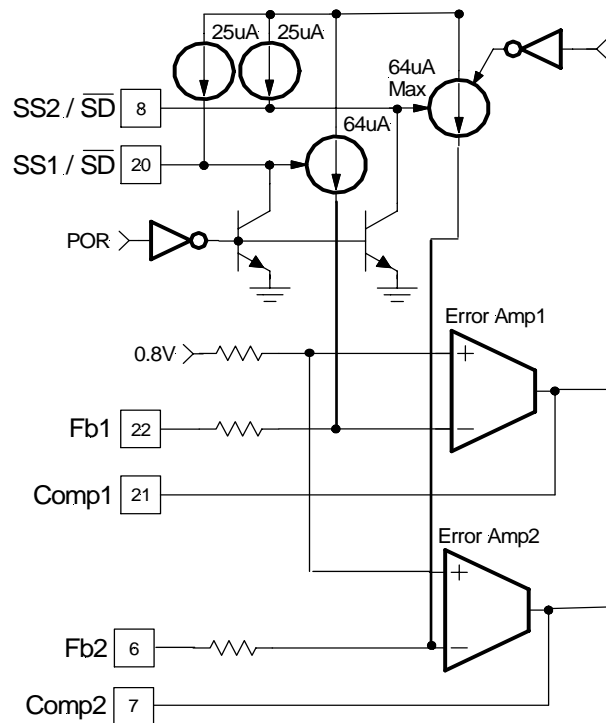
Figure 6 -Soft-start circuit for APU3146X
