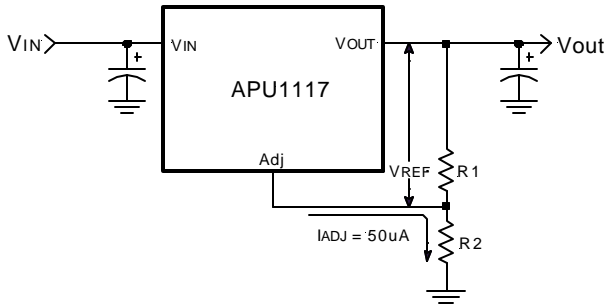
Figure 3 - Typical application of the APU1117 for programming the output voltage.
